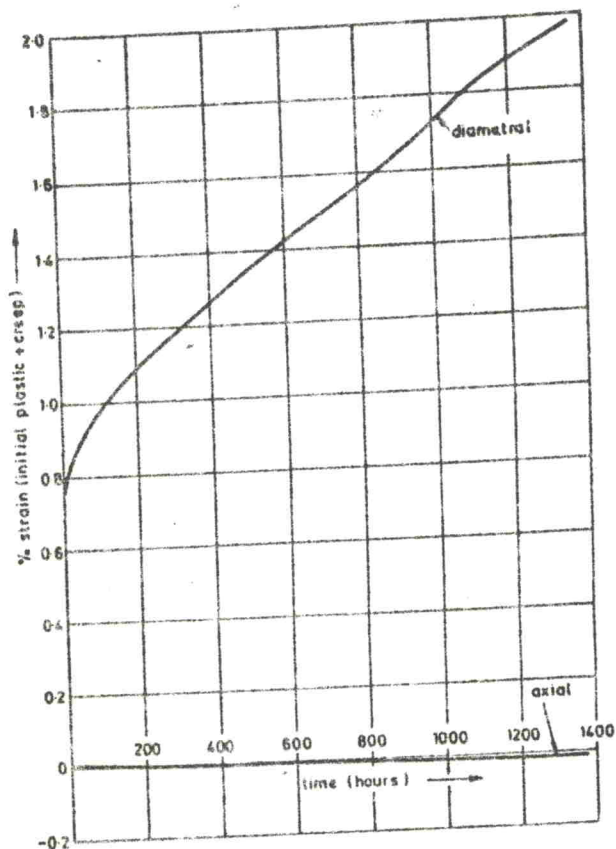
FIG. 1 PRESSURE CREEP TEST ON EN 25 STEEL CYLINDER ( K=1.67 ), TEST PRESSURE 26 ton-ft/in. 2 , TEST TEMPERATURE 350°C
